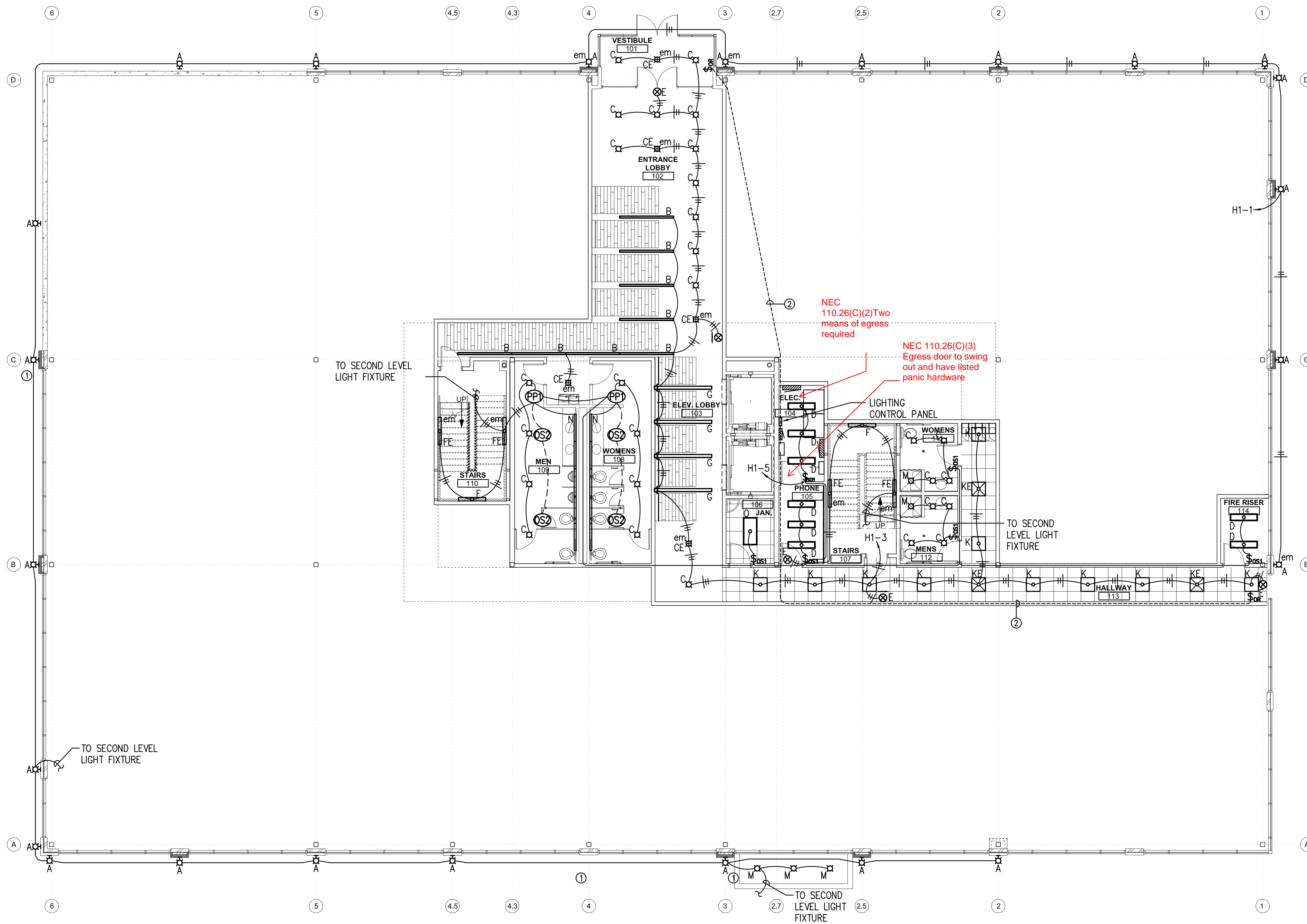
1 E1.1 FIRST FLOOR LIGHTING PLAN scale: 1/8" = 1'-0"
